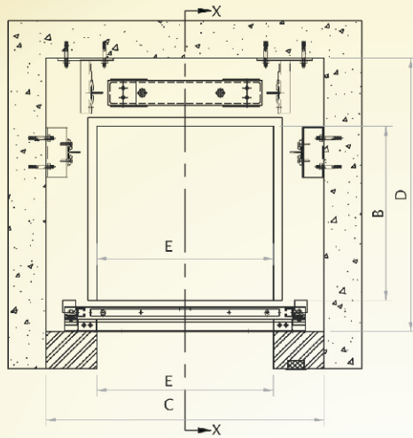
LIFT SHAFT, CAR, C.W. PLAN
