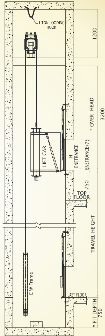
( SECTION : X-X ) LIFT WELL
