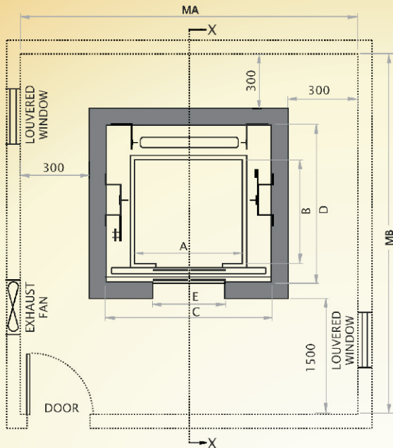
LIFT SHAFT, CAR, C.W. & MACHINE ROOM PLAN
