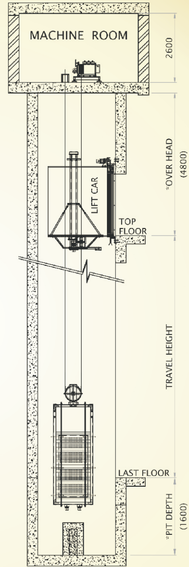
( SECTION : X-X ) LIFT WELL
