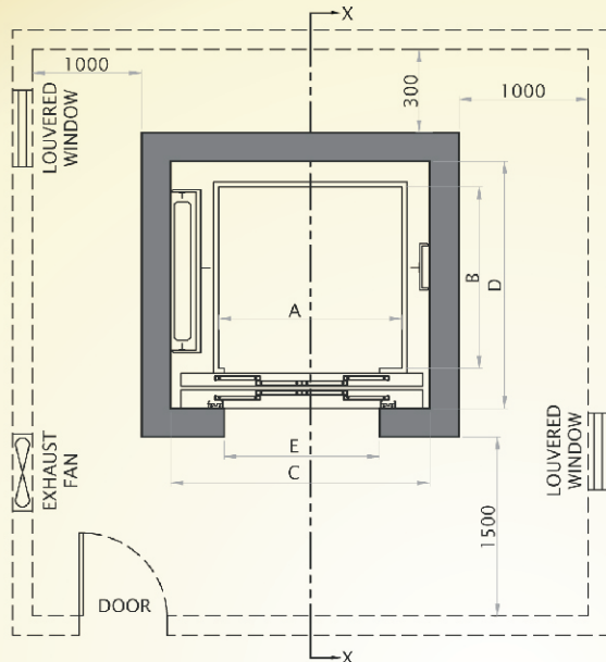
LIFT SHAFT, CAR, C.W. & MACHINE ROOM PLAN
