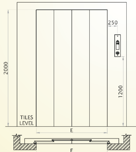
DETAILS AT DOOR OPENING
