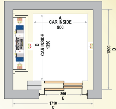
Pit less & specially design for Wheelchair
