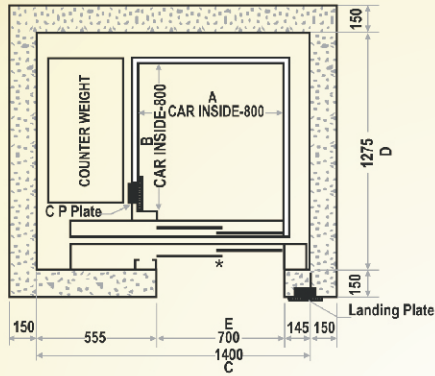
Standard Bungalow Elevator
